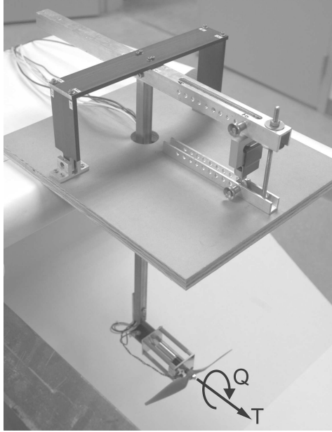
Figure 3. Test apparatus without fairing.
