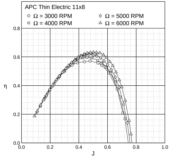
Figure 12. APC Thin Electric 11x8 efficiency curves.
