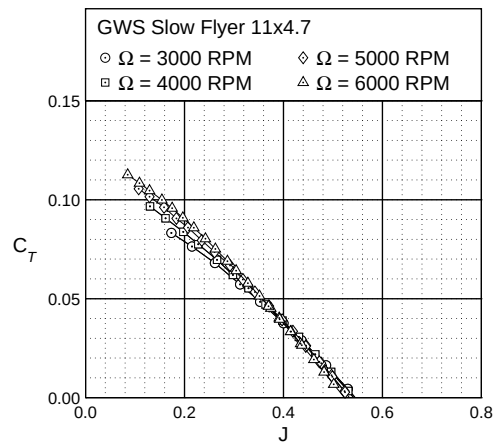
Figure 21. GWS Slow Flyer 11×4.7 thrust characteristics.
