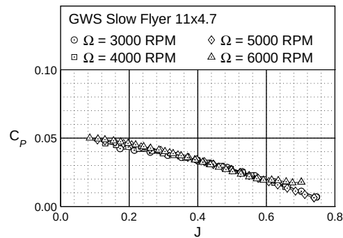
Figure 22. GWS Slow Flyer 11×4.7 power characteristics.
