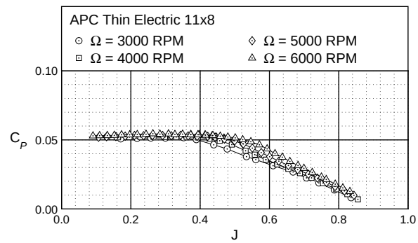
Figure 14. APC Thin Electric 11x8 power characteristics.
