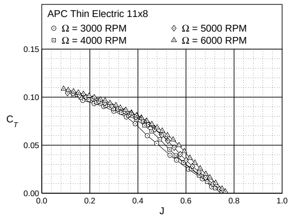
Figure 13. APC Thin Electric 11x8 thrust characteristics.
