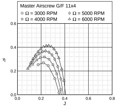
Figure 24. Master Airscrew G/F 11×4 efficiency curves.
