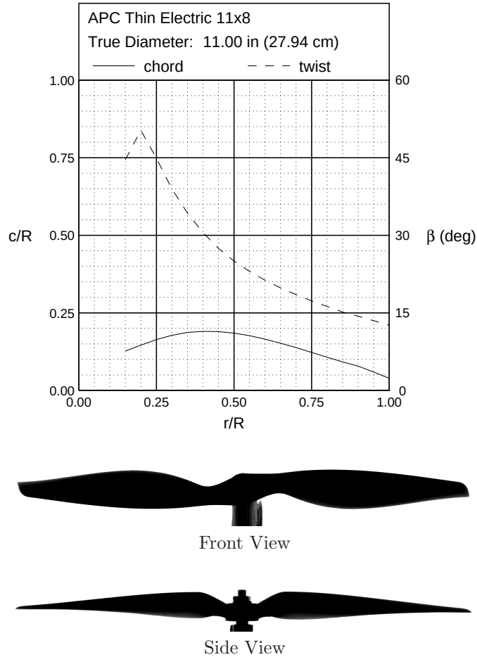
Figure 11. APC Thin Electric 11×8 geometric characteristics.
