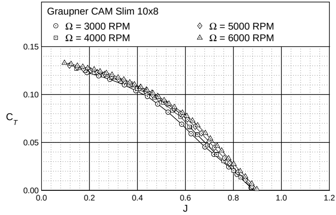
Figure 17. Graupner CAM Slim 10×8 thrust characteristics.
