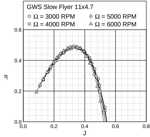
Figure 20. GWS Slow Flyer 11×4.7 efficiency curves.
