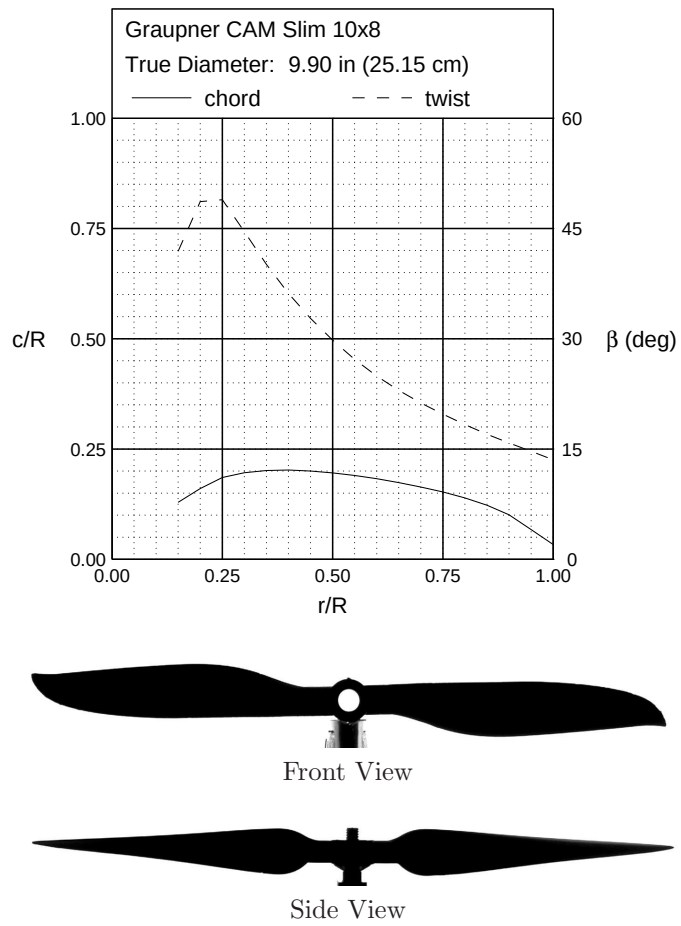
Figure 15. Graupner CAM Slim 10×8 geometric characteristics.
