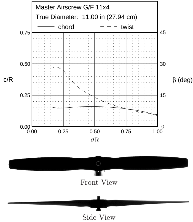
Figure 23. Master Airscrew G/F 11×4 geometric characteristics.
