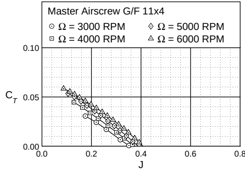
Figure 25. Master Airscrew G/F 11×4 thrust characteristics.
