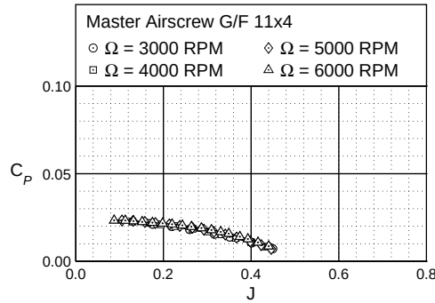
Figure 26. Master Airscrew G/F 11×4 power characteristics.
