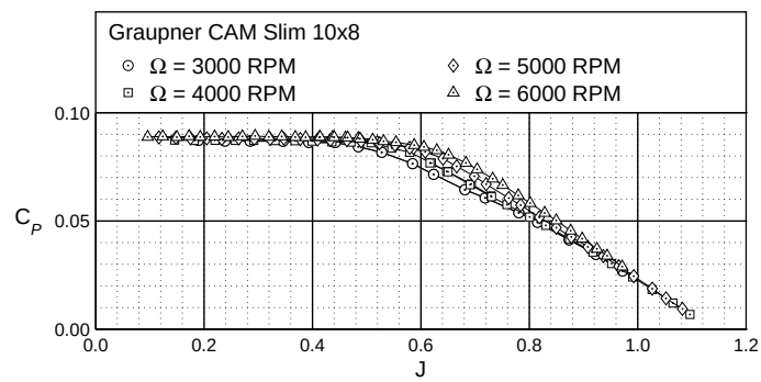
Figure 18. Graupner CAM Slim 10×8 power characteristics.
